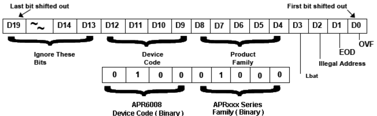
Figure 10 SID Bit Stream
