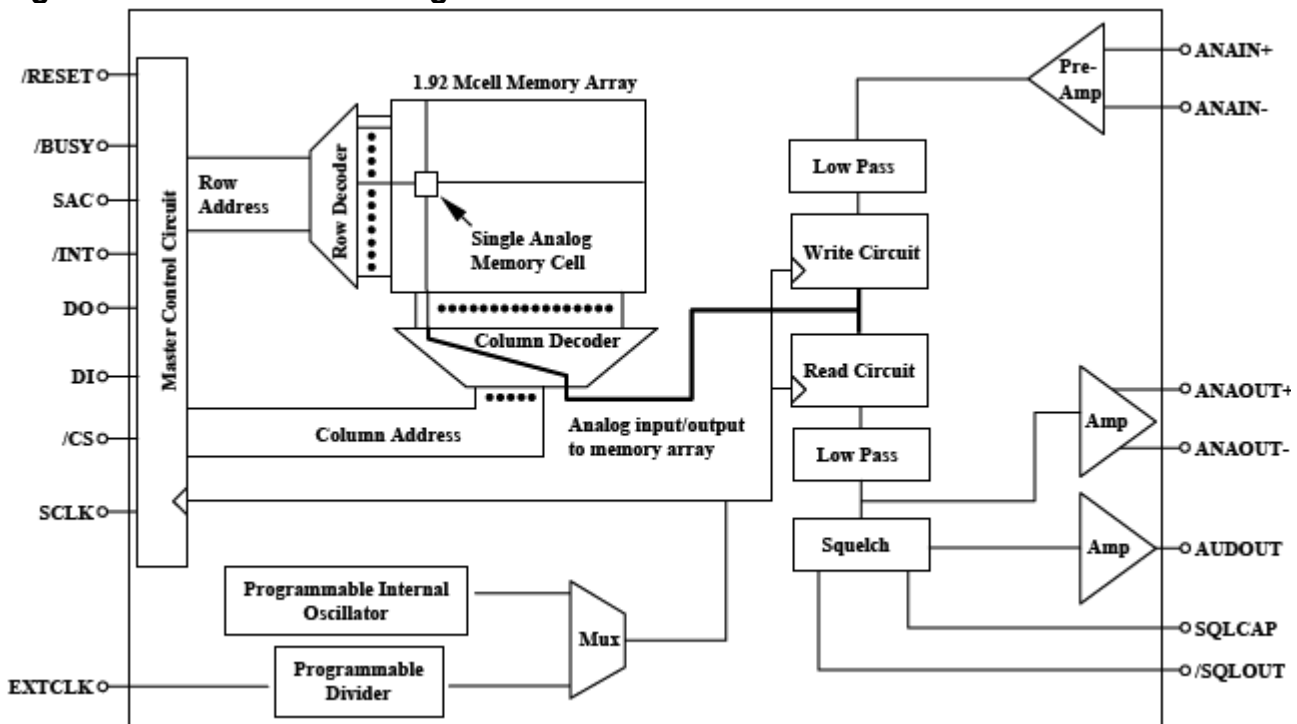
Figure 2 APR6008 Block Diagram :
